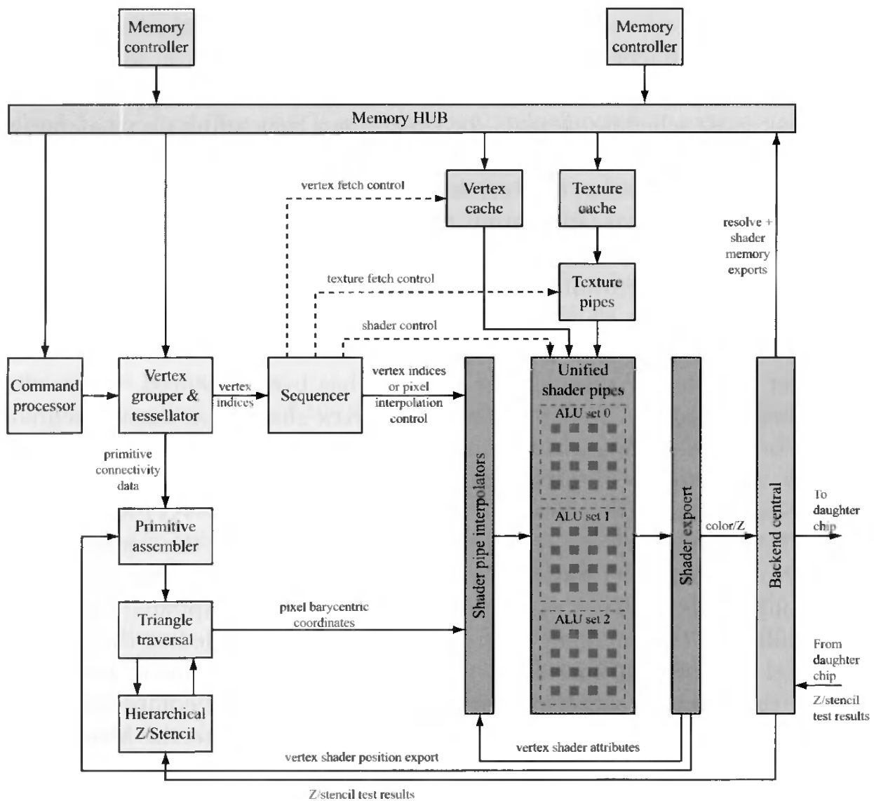
Figure 18.16. Block diagram of the Xbox 360 graphics processor.
